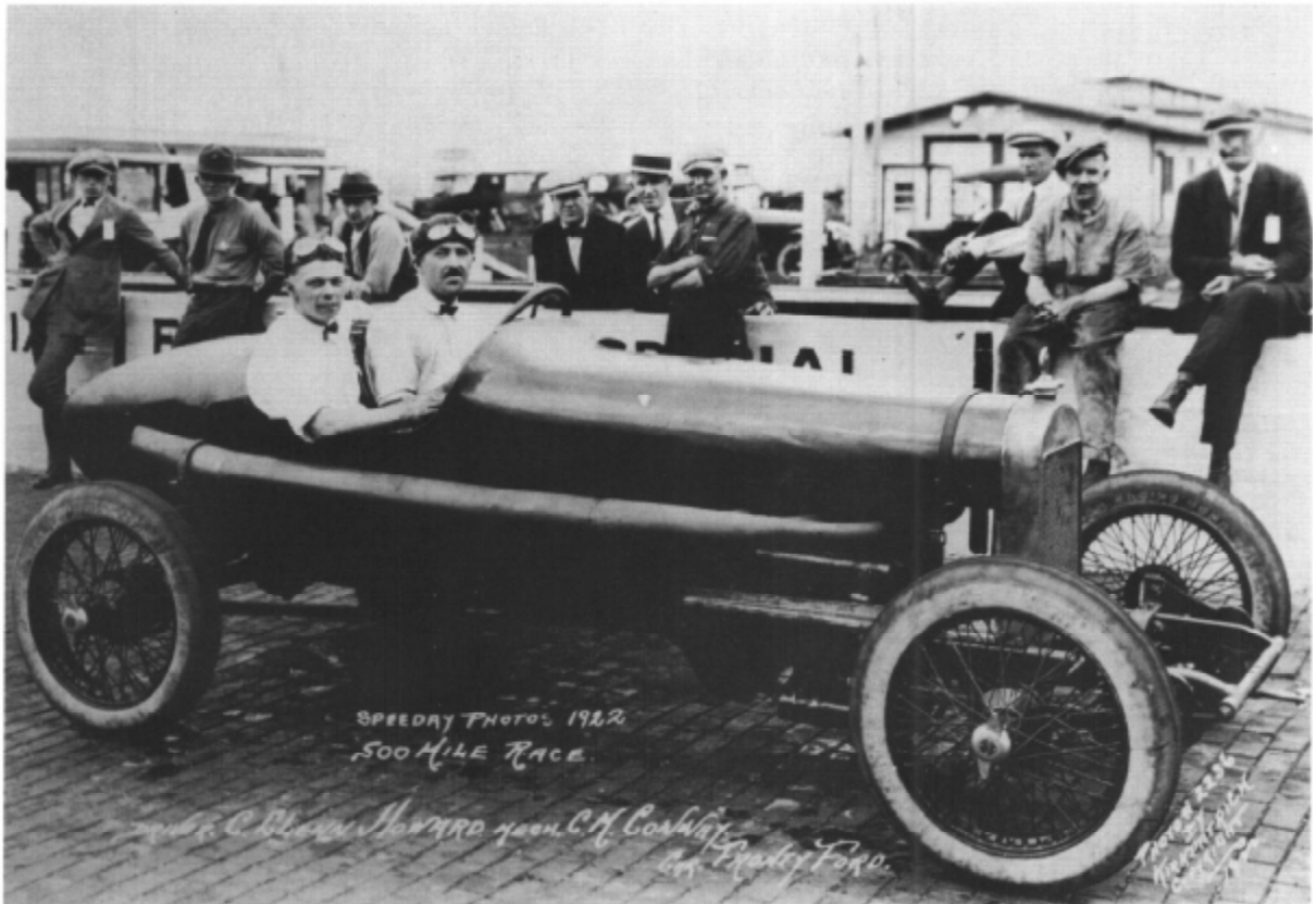
The other Fronty-Ford in the 1922 Indianapolis race was driven by C. Glenn Howard, The mechanic was C. M. Conway, Notice that both of these cars
