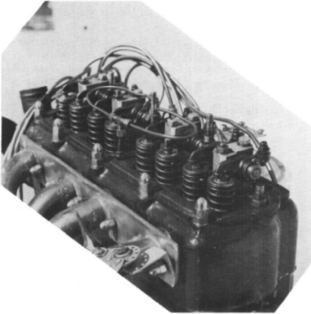
RAJO head as set up for use in a speedster. Engine features pressure lubrication to the rocker arms, as well as internal engine parts. Notice the large oil sump added to the pan; the front plate which drives the water pump and the distributor, and the many other accessories. The engine is owned by R. L, "Doc Pruden, of Santa Monica, Calif,
