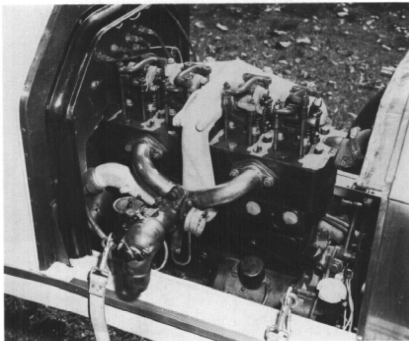
Sixteen valve Roof-Laurel Type B head. Owned by H. D. Thompson, this engine features a Stromberg carburetor (side draft) and apparently is running stock T ignition. These heads, while good performers, were difficult to keep in adjustment because of the valve rocker an construction.
