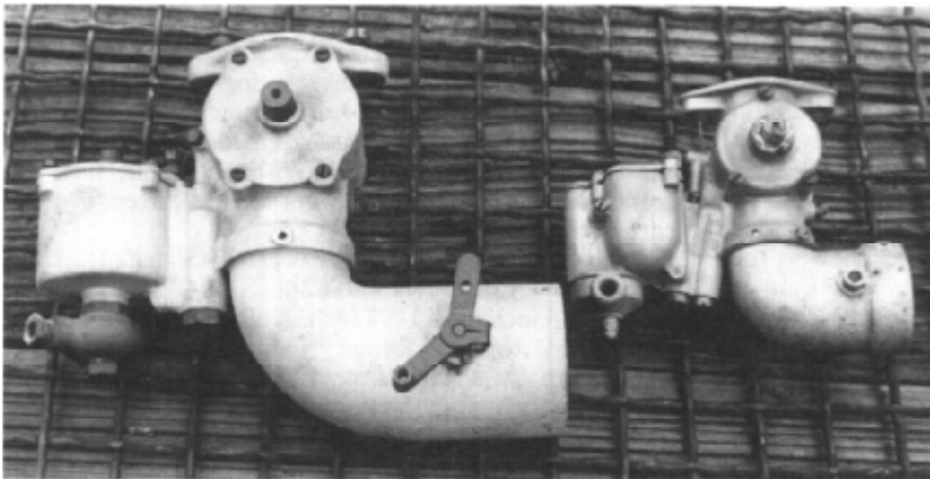
Left. An early large Winfield of non-standard design, perhaps used on a race car. Right is the second type, the Model M. All of the Model M were apparently updraft.
