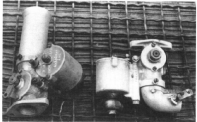
The Model H Winfield side-draft (left) and the Model V updraft carburetors. Both share the same basic design. These are the earliest models.
