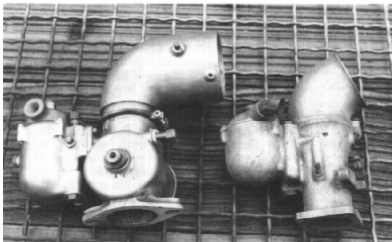
Non-standard Winfield carburetors. The left appears to be a combination of M and S features with the barrel throttle; the right one has the Model S throttle but with an integral float bowl. These appear to both be downdraft, no doubt for race cars.
